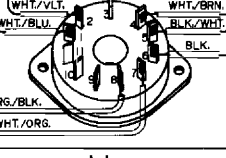
J1 REMO-CON JACK
