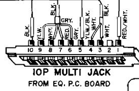
SERVO CONTROL P.C. BOARD TW-1049
