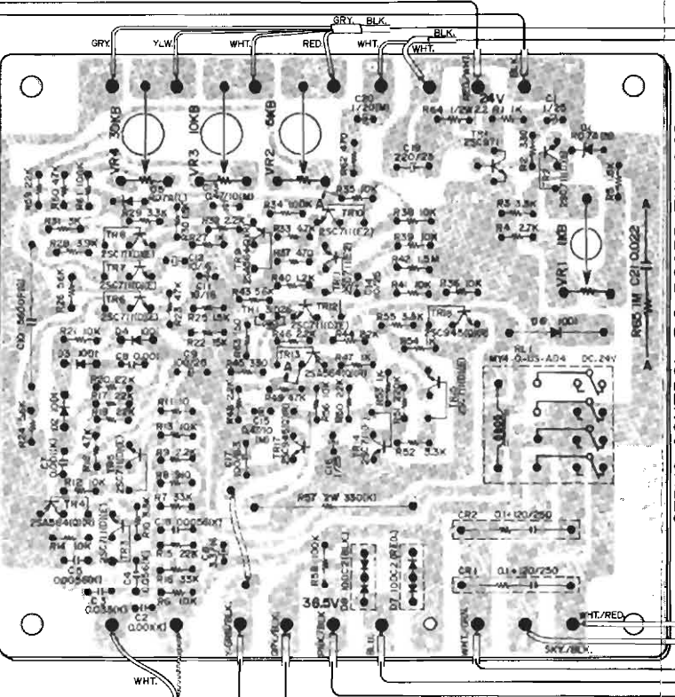
SERVO CONTROL P.C. BOARD TW-1049
