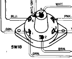
VOLTAGE SELECTOR & FUSE POST
